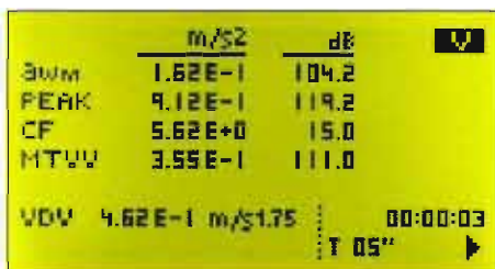
Overall values of acceleration evaluation parameters ISO 2631-2:2003
